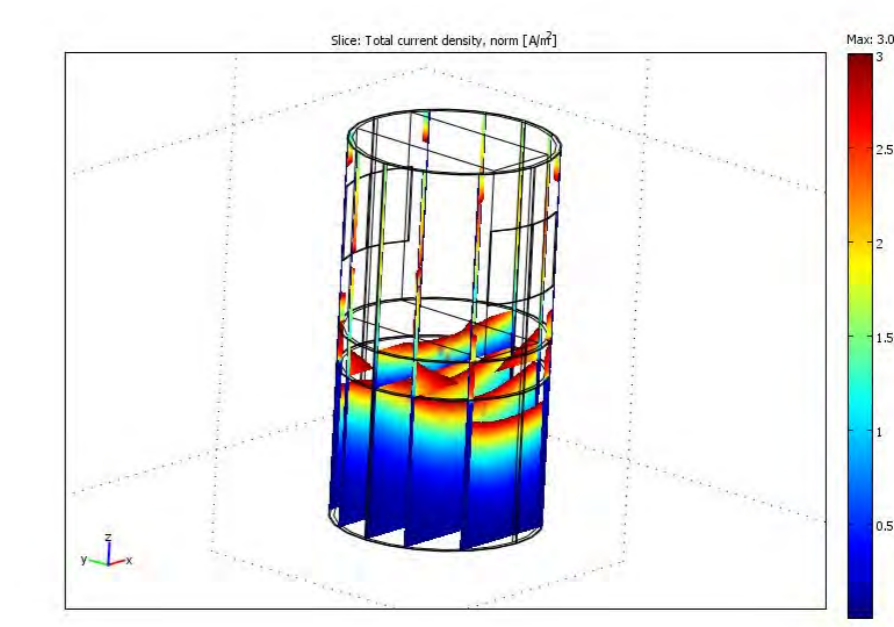
FIGURE 7: Current density at 1KHz
