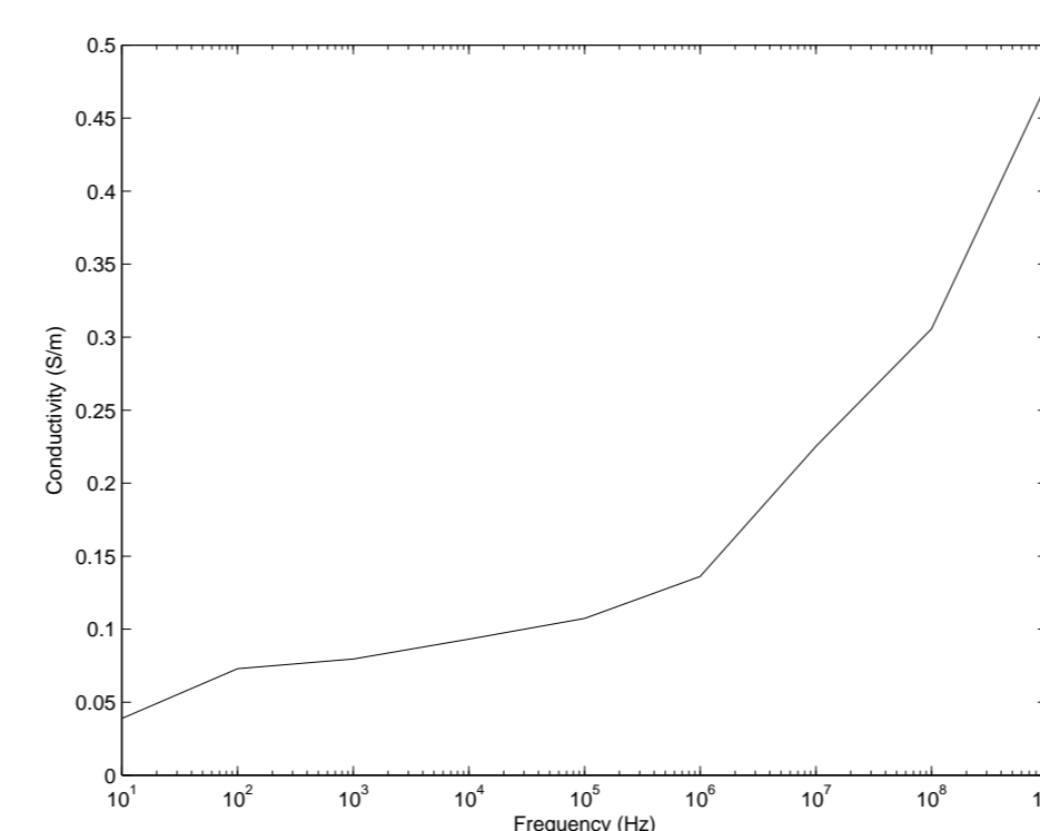
FIGURE 2: Average conductivity of lungs
